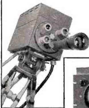
IMAGE ORTHICON PICKUP HEAD
